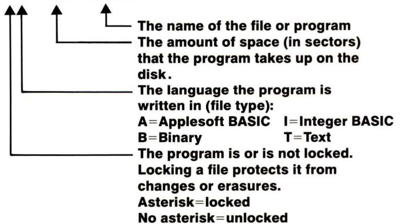
Figure 4-1. Typical Catalog
