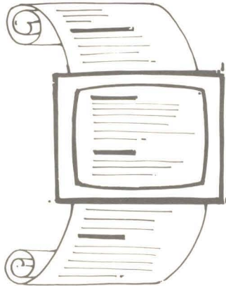
Figure 5-2. Scrolling Window
