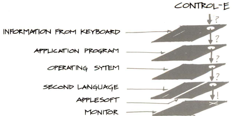
Figure 5-1. Command "Filters"
